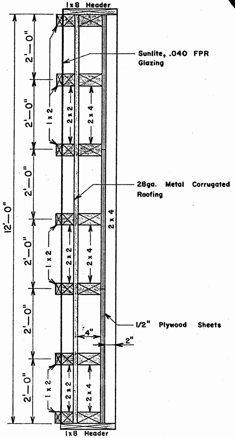
COLLECTOR'S SECTION A-A
