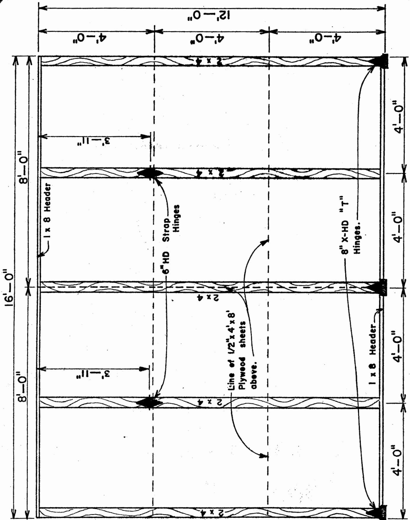
REAR VIEW & FRAMING OF COLLECTOR
